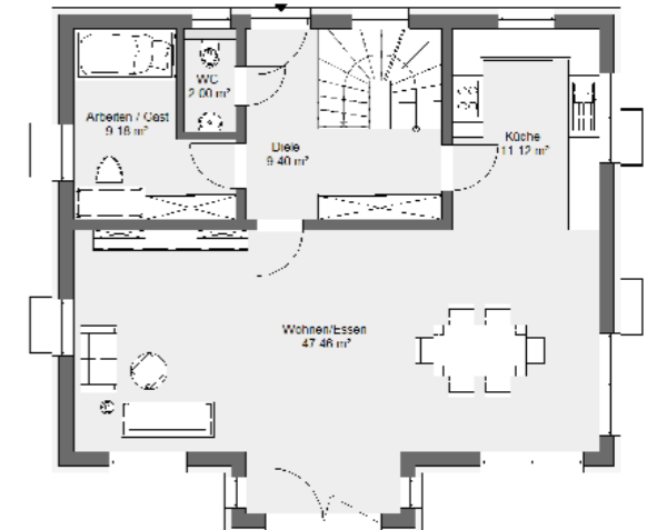
Erdgeschossvariante
